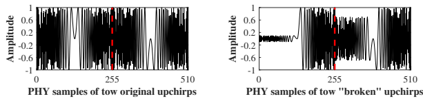
(a) original up-chirps. (b) broken up-chirps.
