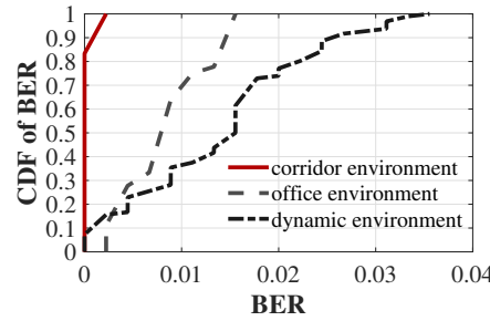
Fig. 20. BER of covert channel under various environments.
