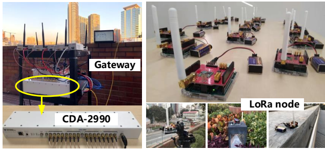
Figure 12: PCube implementation.
