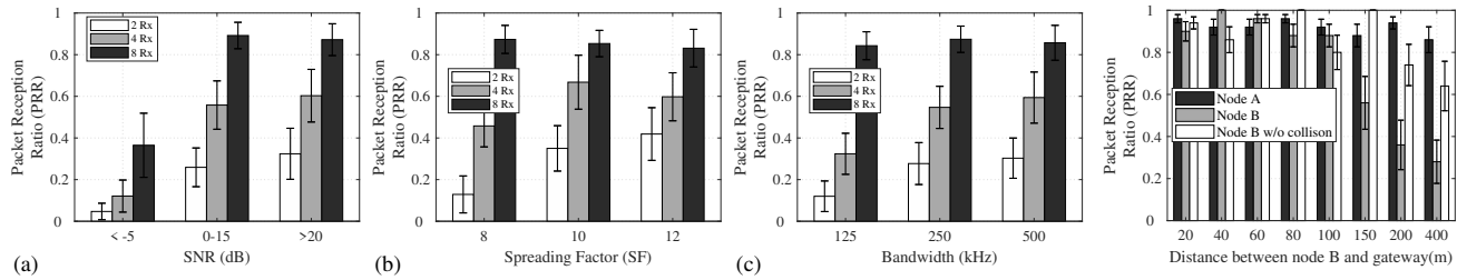
Figure 18: Impacts of (a) SNR (b) spreading factor and (c) bandwidth on PCube when decoding 20 concurrent packets.
